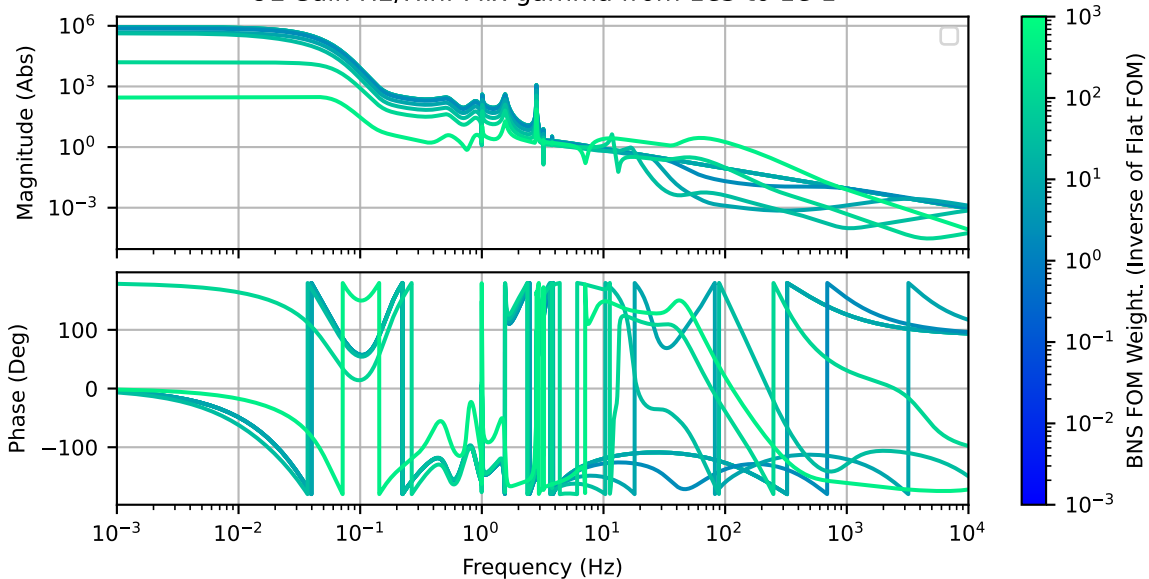
OL Gain H2/Hinf Mix gamma from 1e3 to 1e-1
