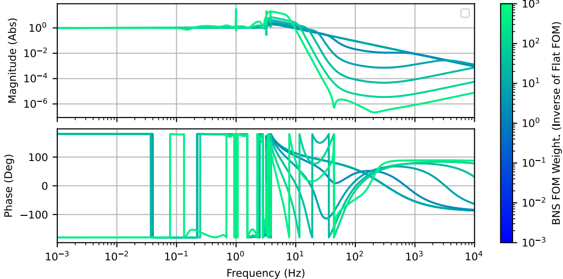
CL Gain H2/Hinf Mix gamma from 1e3 to 1e-1
