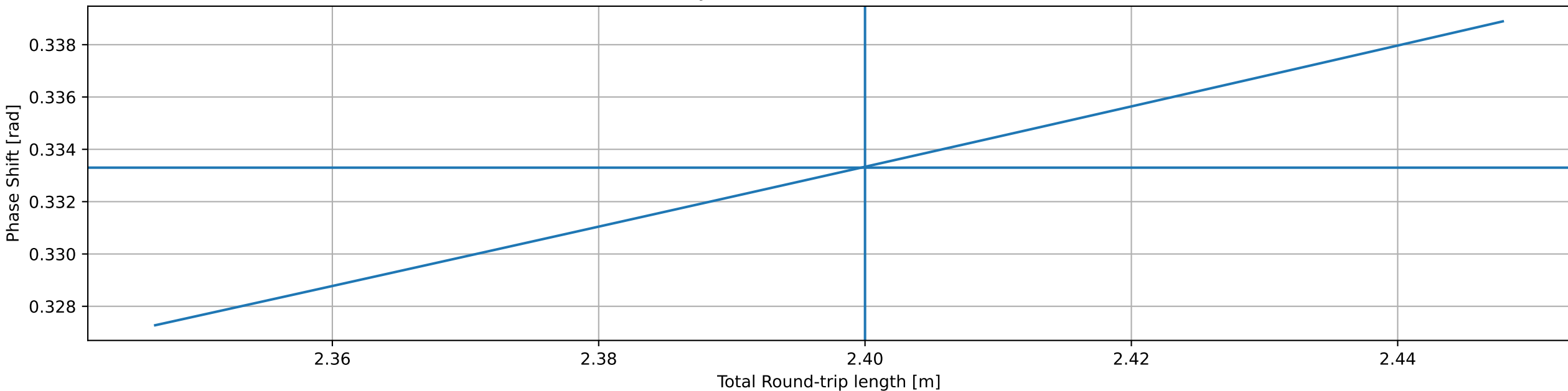
Fractional RT Gouy Phase With 1 Curved Mirror of 1.60m ROC
