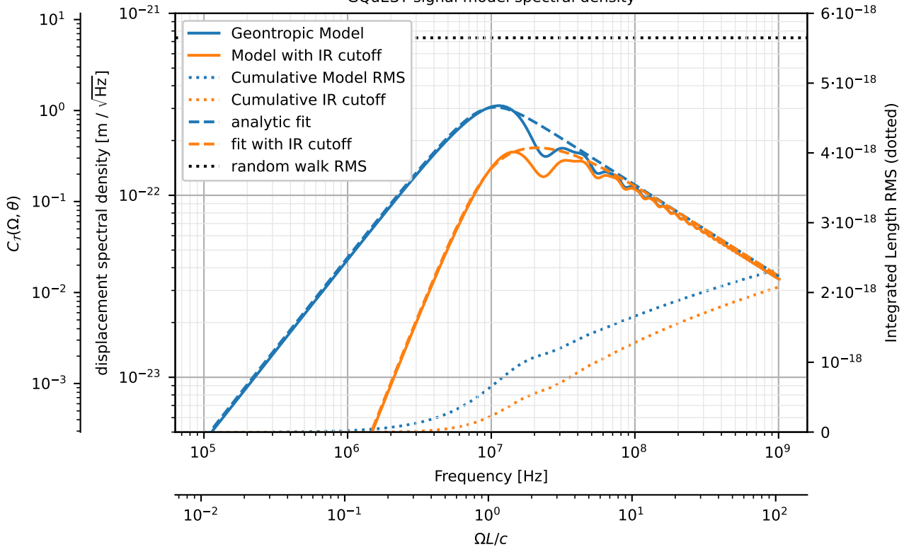
GQuEST signal model spectral density
