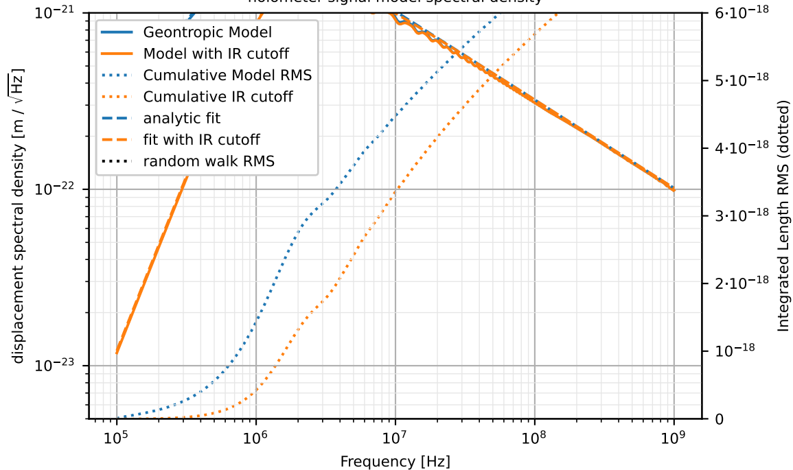
holometer signal model spectral density
