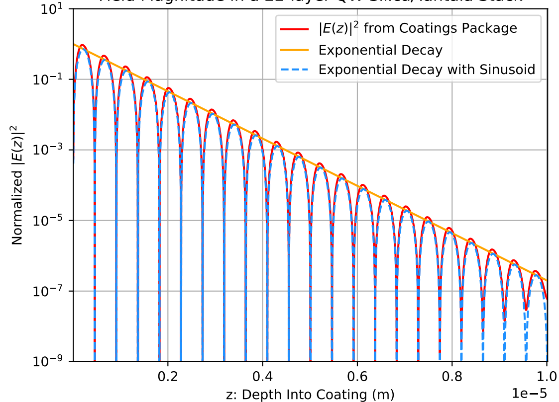
Field Magnitude in a 22-layer QW Silica/Tantala Stack
