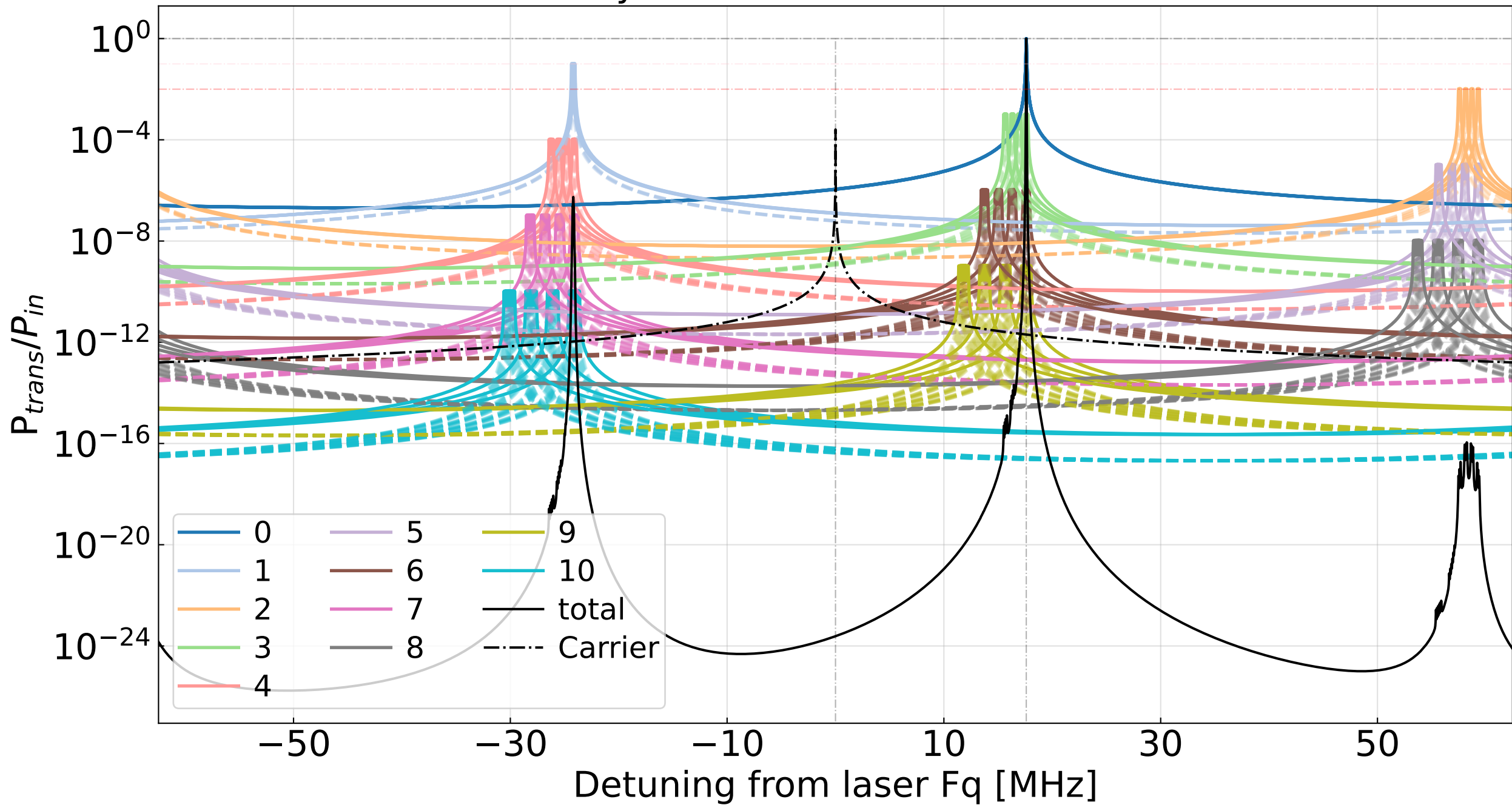
Cavity Transmission with 4 cavities
