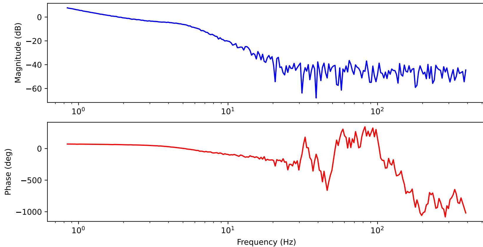
Open Loop Gain Transfer Function (CP)
