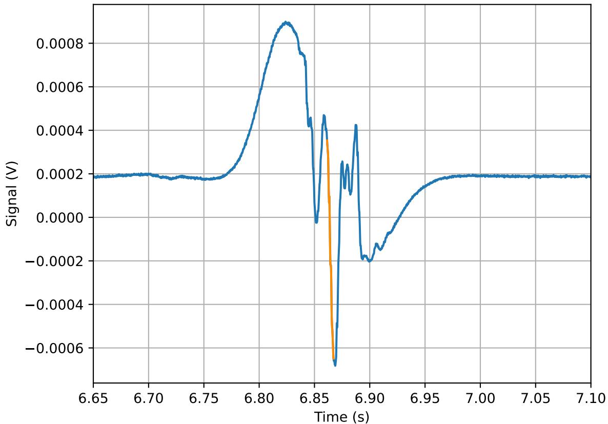
Error Signal (probe with pump)
